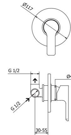
2V030 Complete concealed shower mixer
