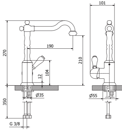
93361 Wash basin mixer lateral lever
