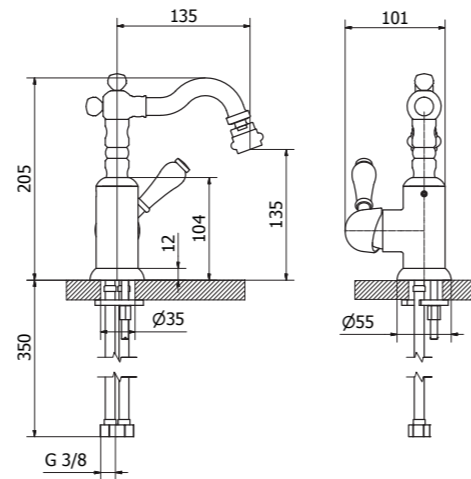
93461 Bidet mixer lateral lever
