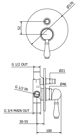
93050 Complete concealed bath-shower mixer
