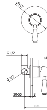
93030 Complete concealed shower mixer
