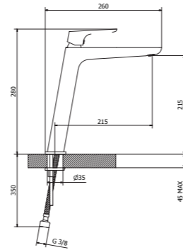
SW721 High wash basin mixer
