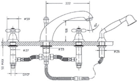
58154 Deck mounted bath mixer
