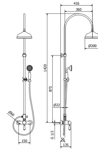
15342 Shower column with jar shower mixer
