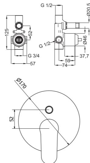
2R050 Concealed bath shower mixer
