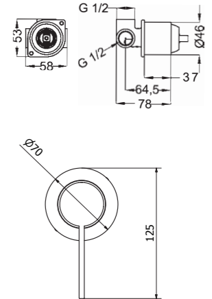
2H030 Concealed shower mixer
