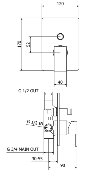
4L050 Concealed bath-shower mixer
