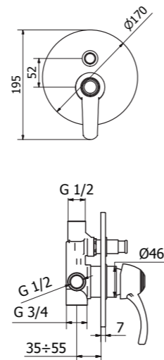
94050 Concealed bath-shower mixer
