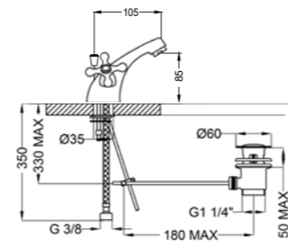
6214E One hole wash basin mixer
