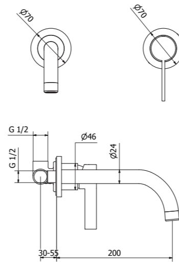
2H692 Wall mounted basin mixer 2 pcs.
