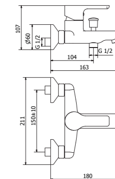
2V545 Vertical bath mixer
