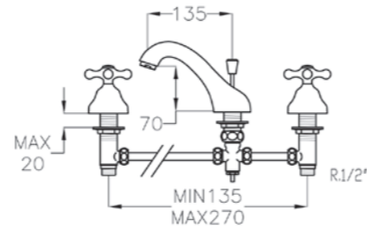
6613E 3 holes wash basin mixer
