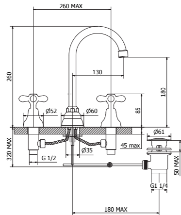
6613E 3 holes wash basin mixer
