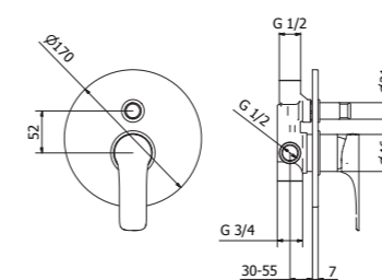
2V050 Concealed bath-shower mixer
