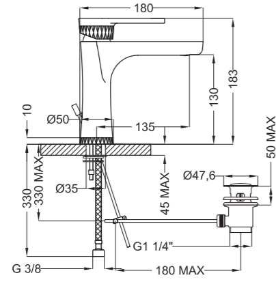
2J710 Wash basin mixer
