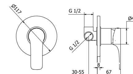
2V030 Concealed shower mixer
